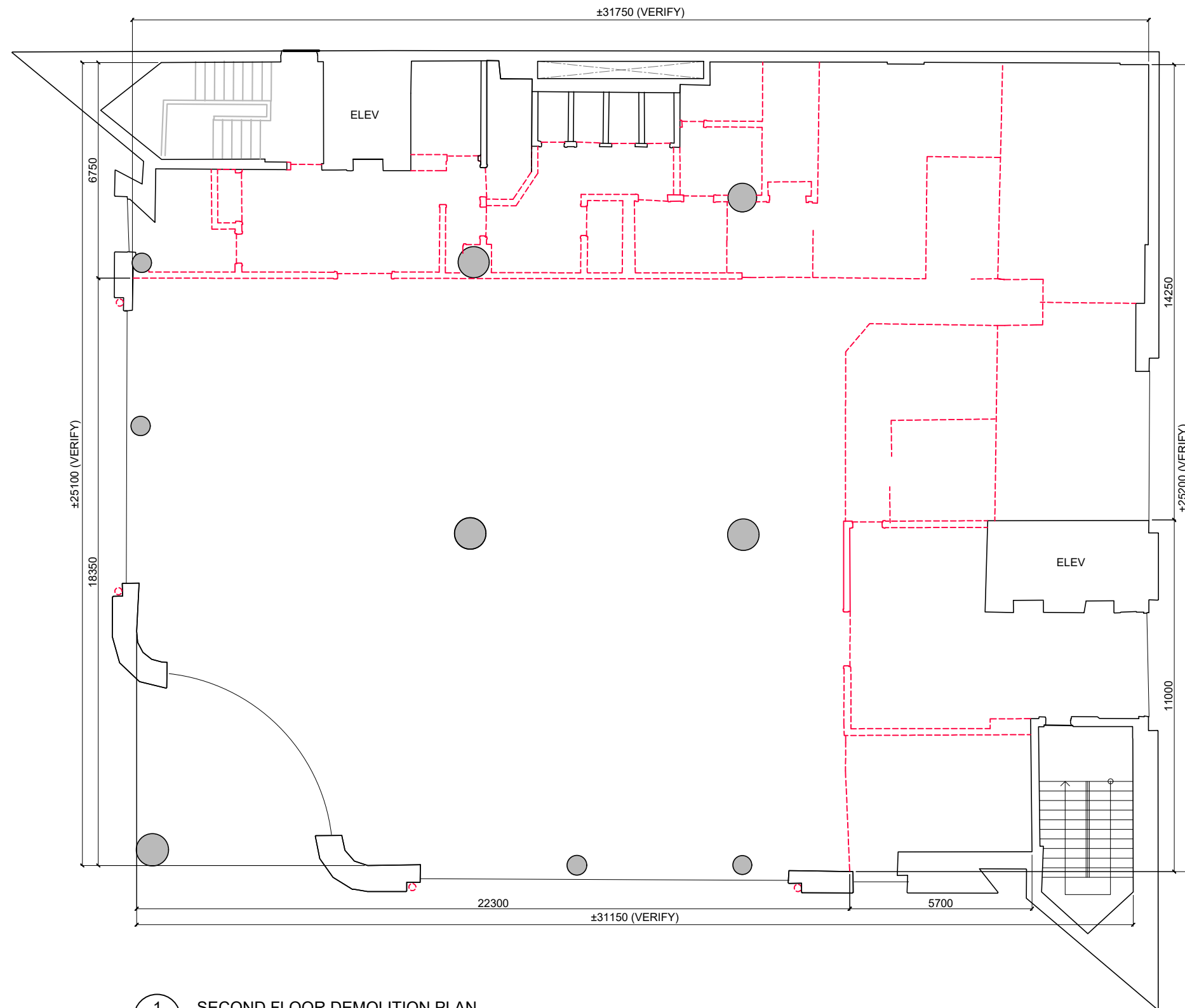
1 SECOND FLOOR DEMOLITION PLAN I-009b SCALE 1:150
